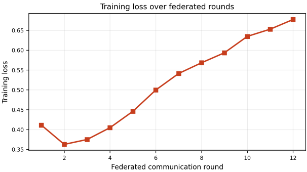
Figure 6. Training-loss trace over communication rounds generated from validation_history.csv. Non-monotonic behavior is expected in heterogeneous federated learning and should be interpreted together with validation metrics.
