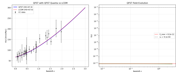
Figure 1. Background evolution in QFST. (i) H(z) compared with \Lambda CDM and Cosmic Chronometer data. (ii) The numerical solution for \tilde{\nu}(z) used to reconstruct \Omega_{DE}(z) .
