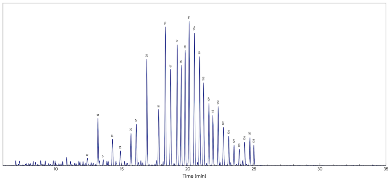
Figure 3. Total ion chromatogram (TIC) of the resinous bioactive fraction (E5) obtained by GC-MS analysis.
